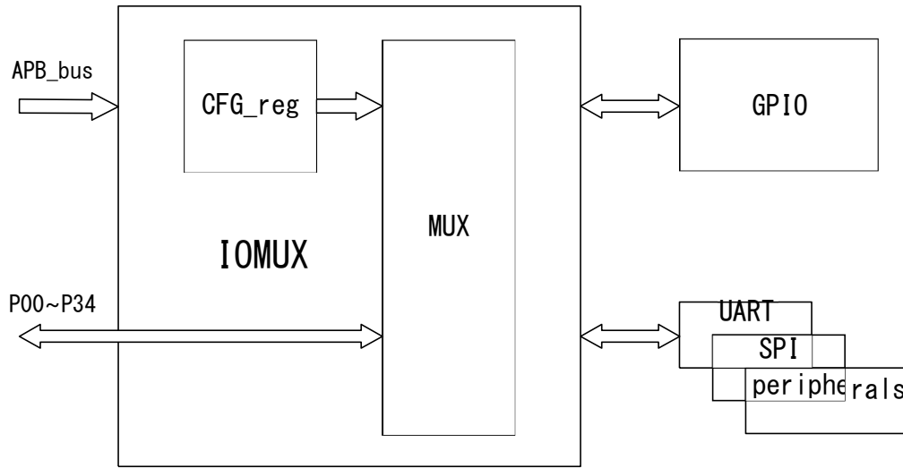
Figure 11: IOMUX structure diagram
