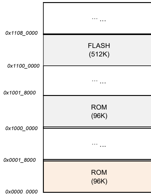
Figure 4: BT1681 boot mode
