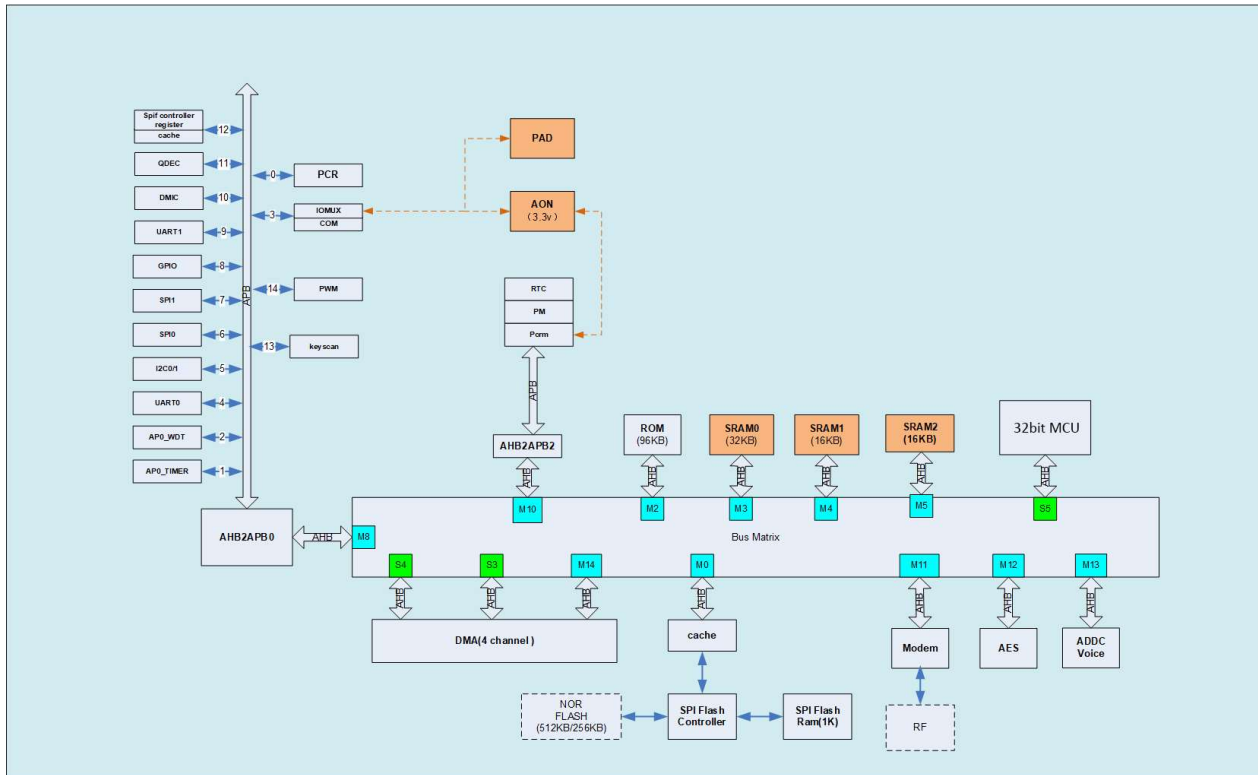
Figure 1: BT1681 block diagram
