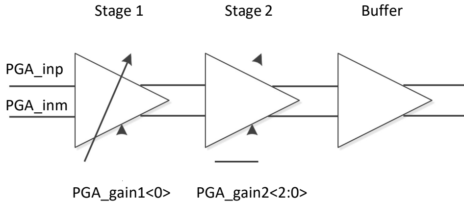
Figure 17: PGA path
