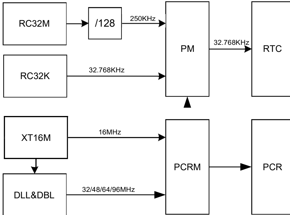
Figure 9: Clock management
