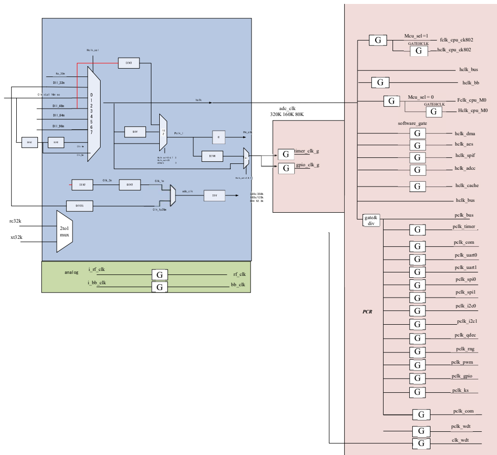
Figure 10: Clock structure diagram
