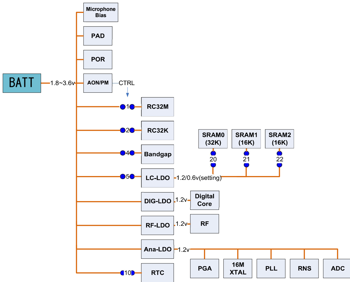
Figure 7: Power system
