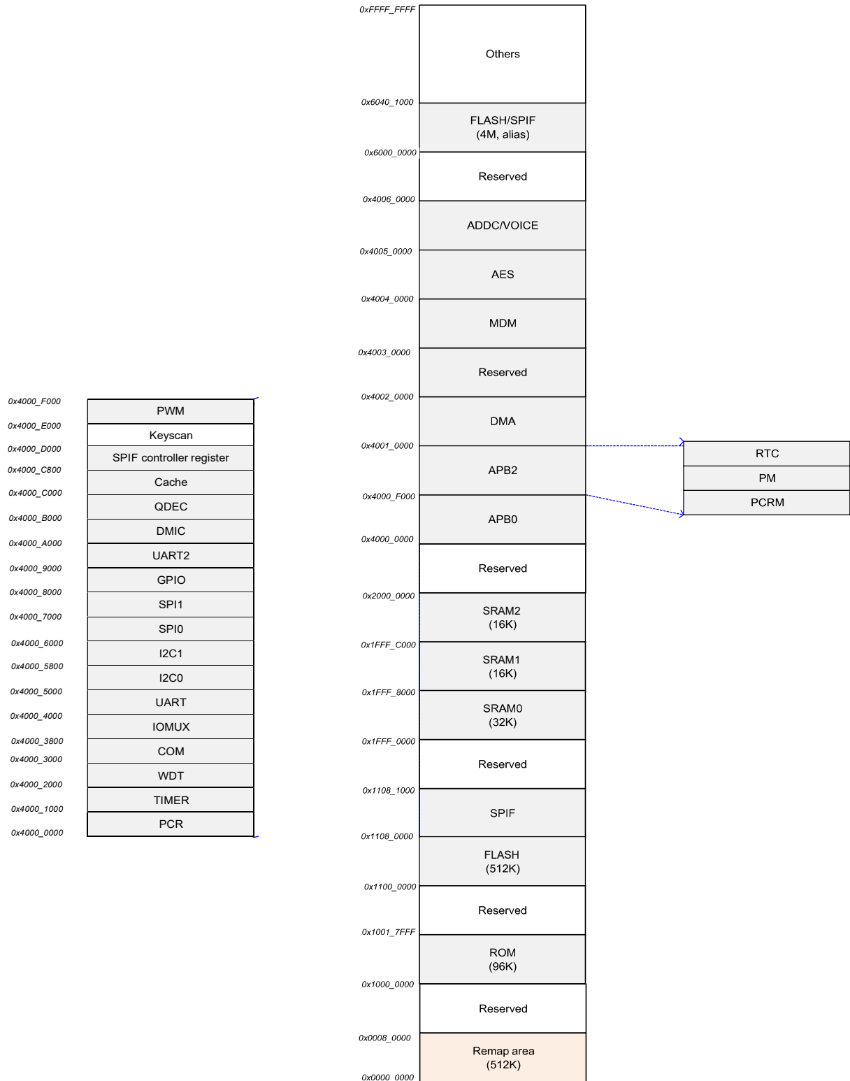
Figure 3: BT1681 memory space
