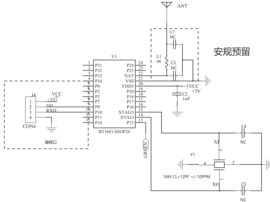
Figure 21: Sample application of SSOP24
