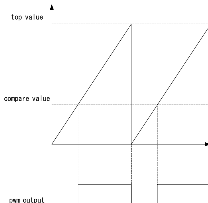
Figure 15: PWM operation
