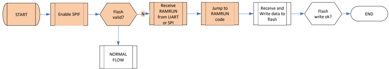
Figure 5: Bootloader flow
