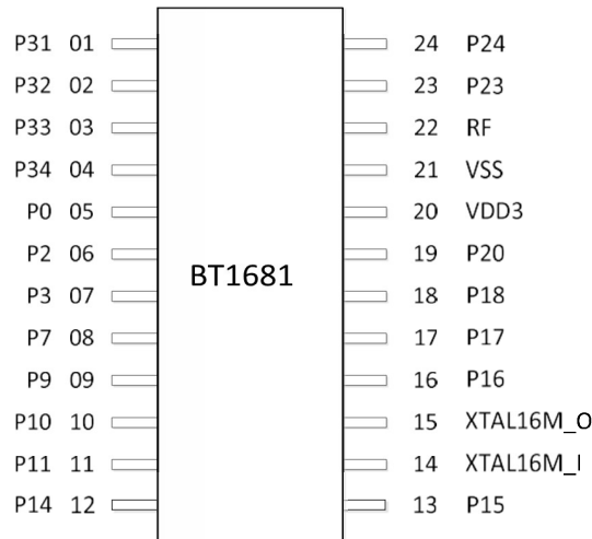
Figure 2: Pin assignment – BT1681 SSOP24 package
