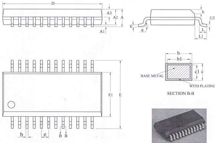
Figure 20: SSOP24 package dimensions
