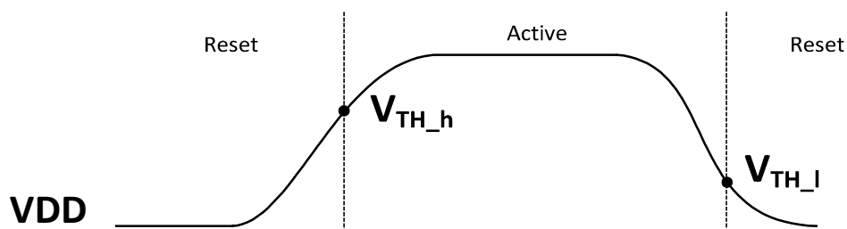
Figure 8: UVLO reset
