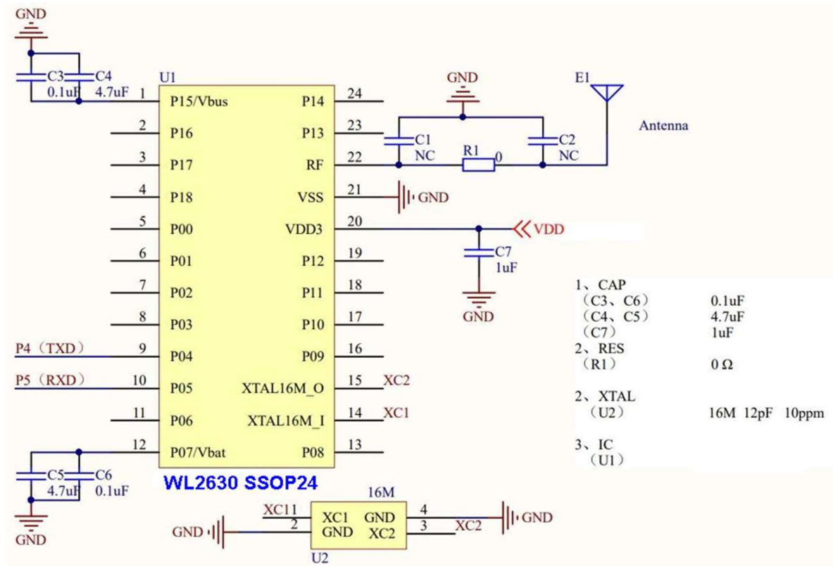
Figure 25: Sample Application of SSOP24
