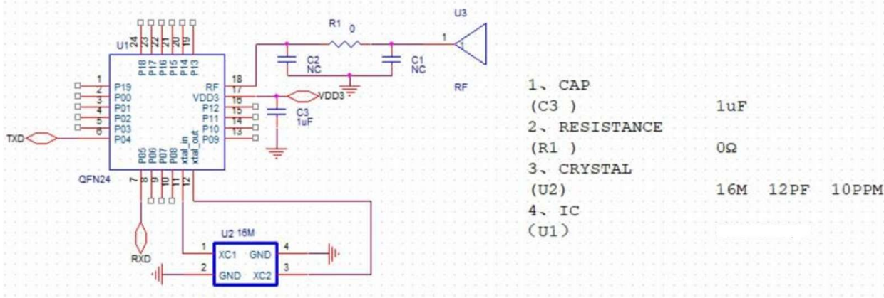
Figure 29: Sample application of WL2630 QFN24
