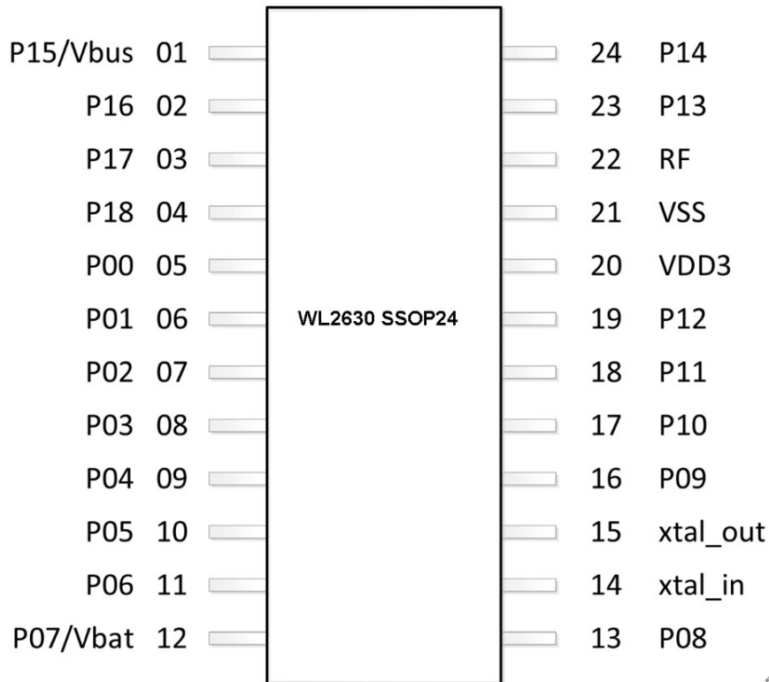
Figure 2: Pin assignment – WL2630 SSOP24 package
