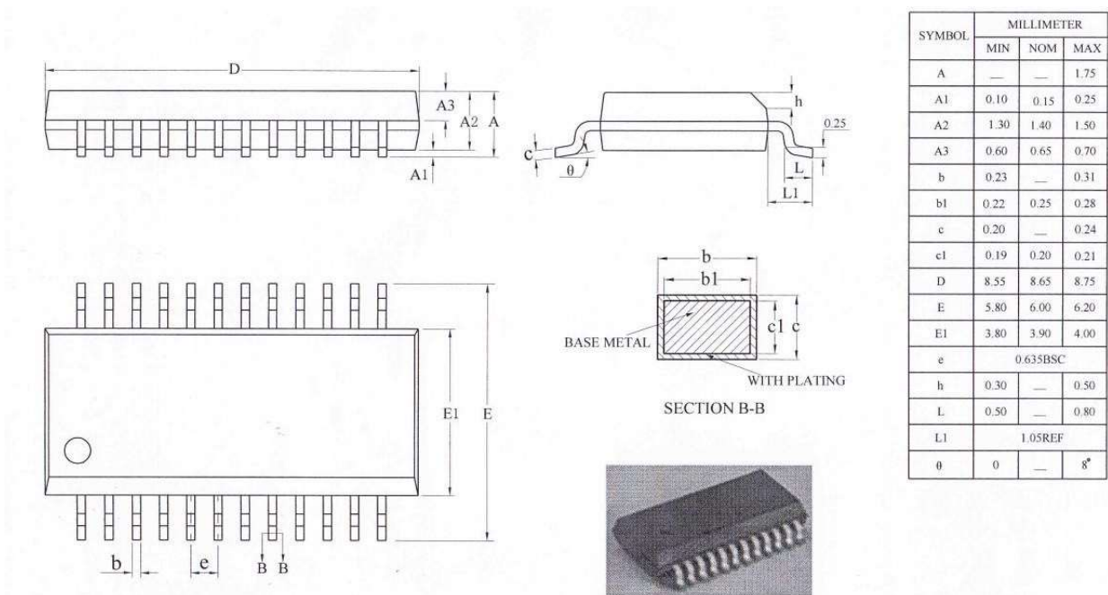
Figure 19: SSOP24 Package Dimensions
