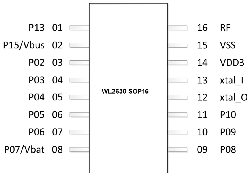
Figure 3: Pin assignment – WL2630 SOP16 package
