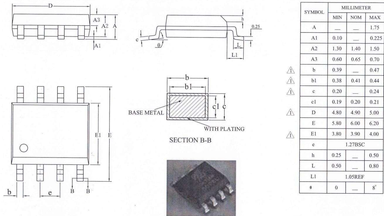
Figure 22: SOP8 Package Dimensions
