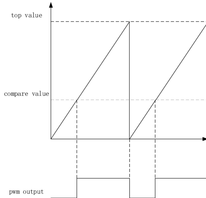
Figure 15: PWM operation
