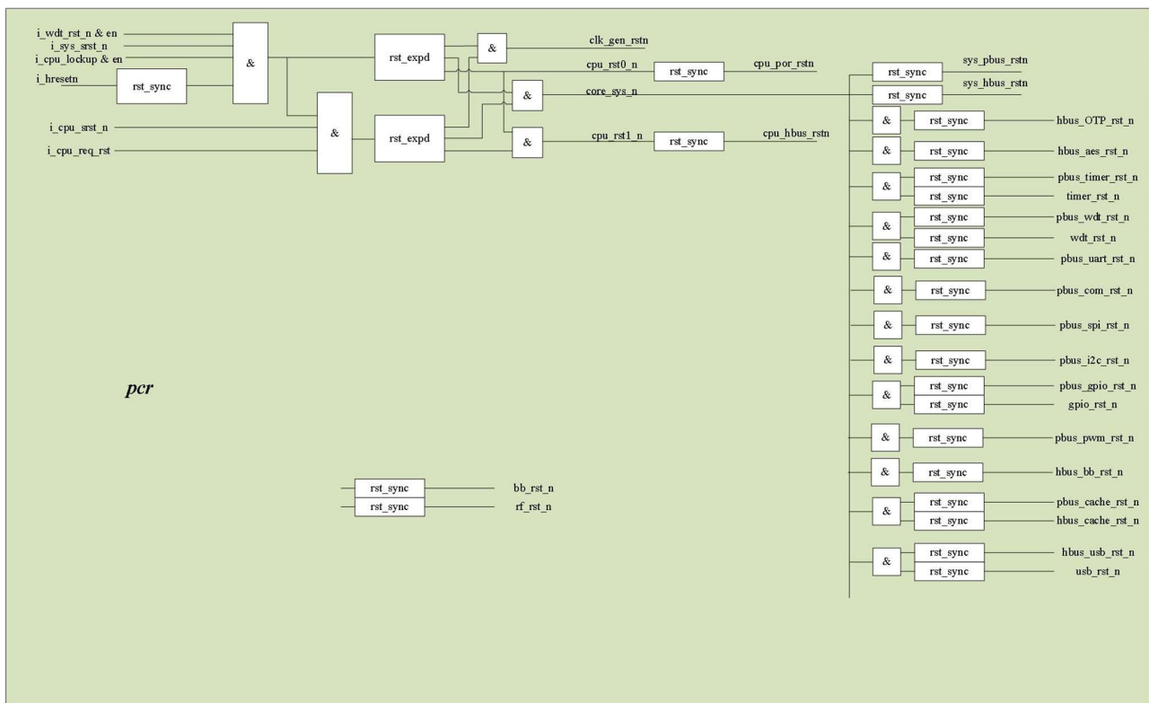
Figure 9: WL2630 power, clock and reset
