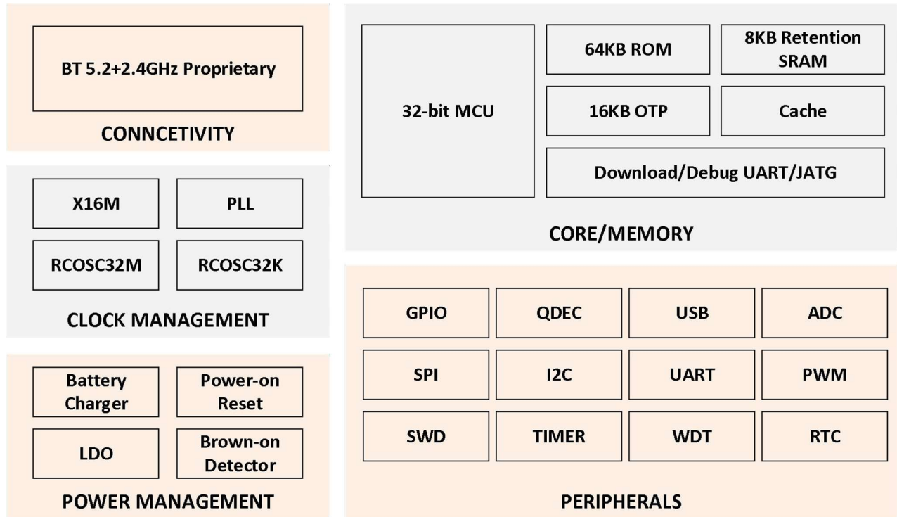
Figure 1: WL2630 Block Diagram
