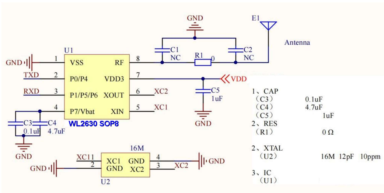
Figure 27: Sample Application of SOP8
