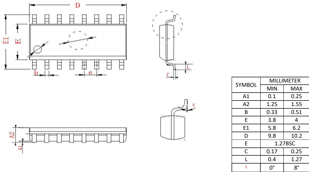
Figure 20: SOP16 Package Dimensions
