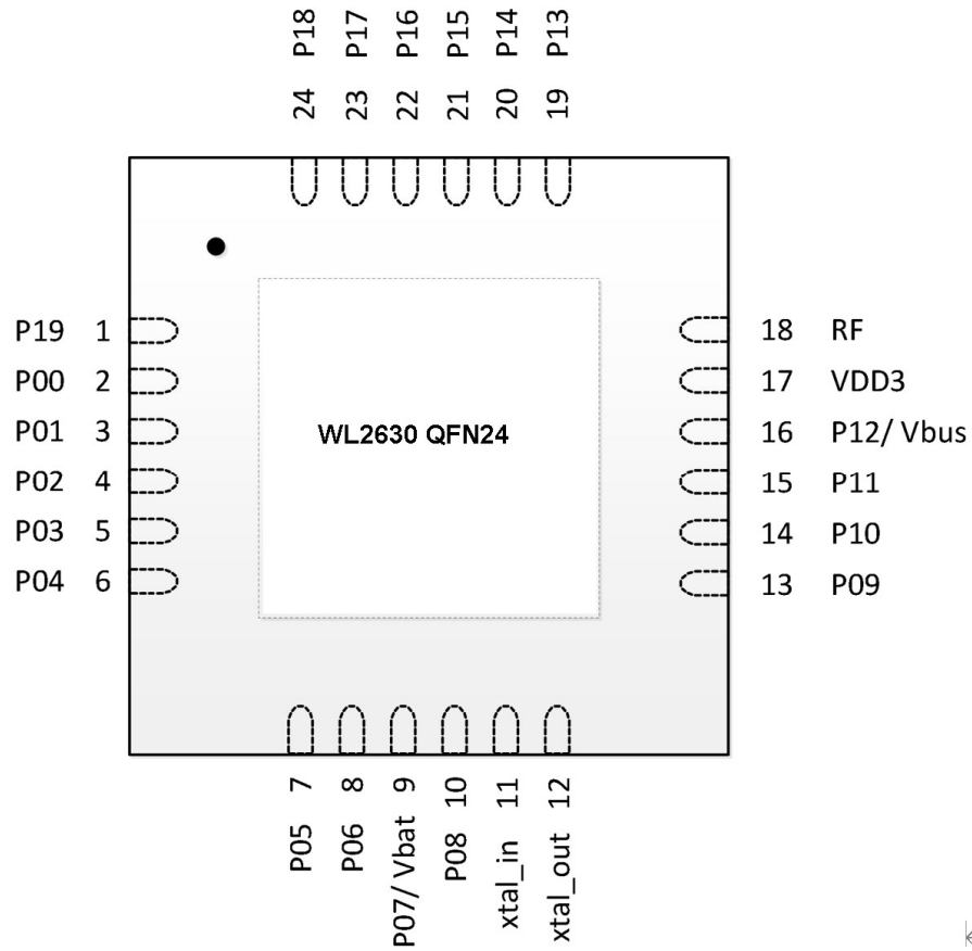
Figure 6: Pin assignment – WL2630 QFN24 package
