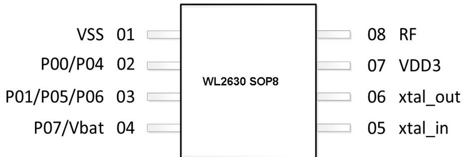
Figure 4: Pin assignment – WL2630 SOP8 package
