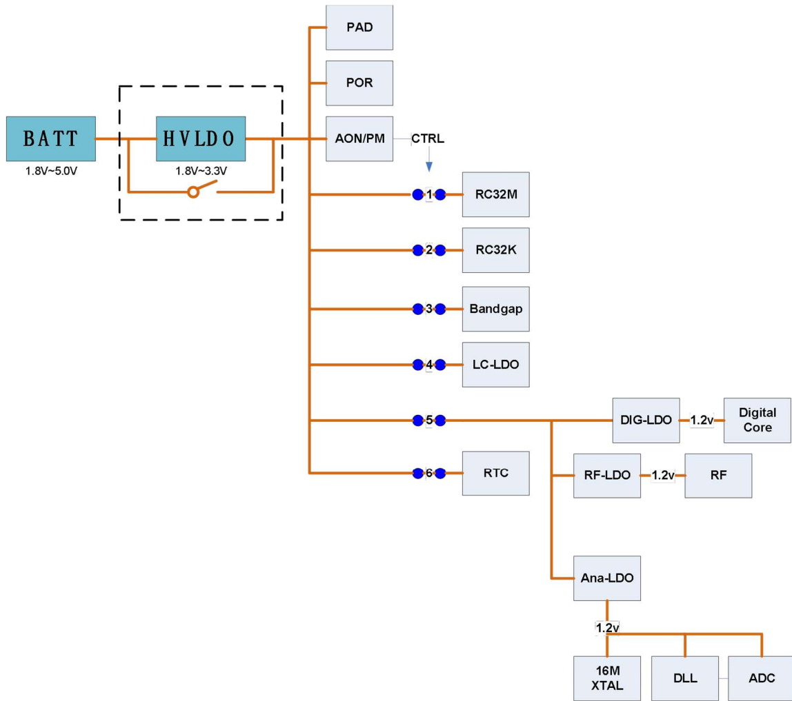
Figure 10: Power system
