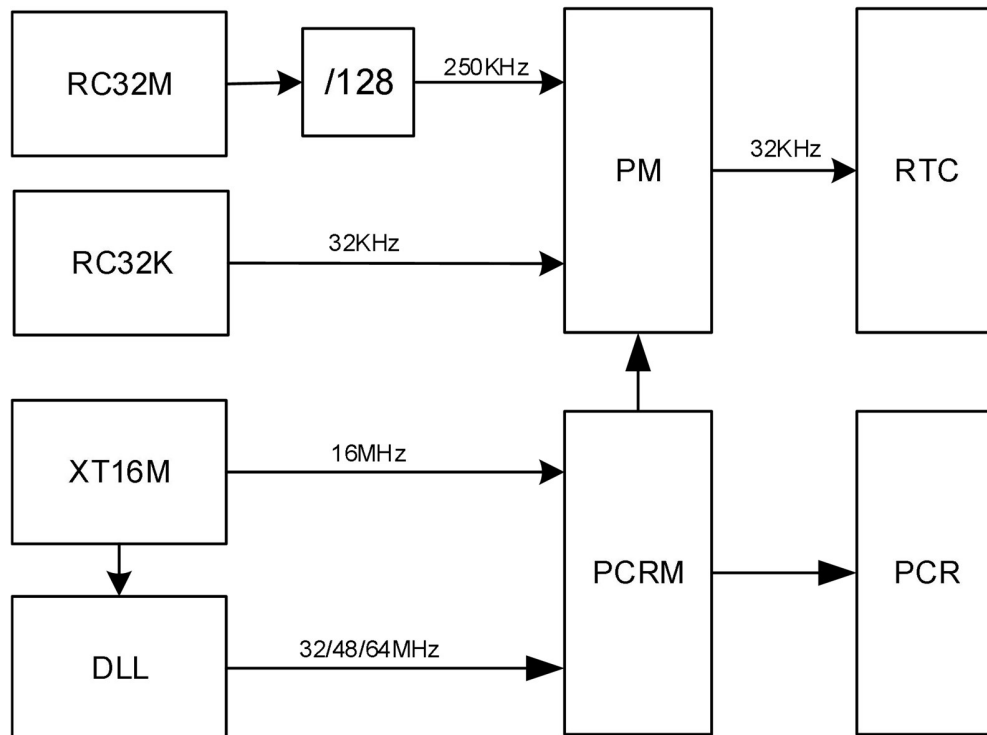
Figure 12: Clock management
