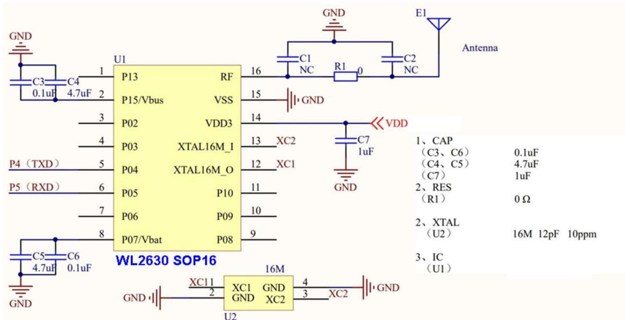
Figure 26: Sample Application of SOP16
