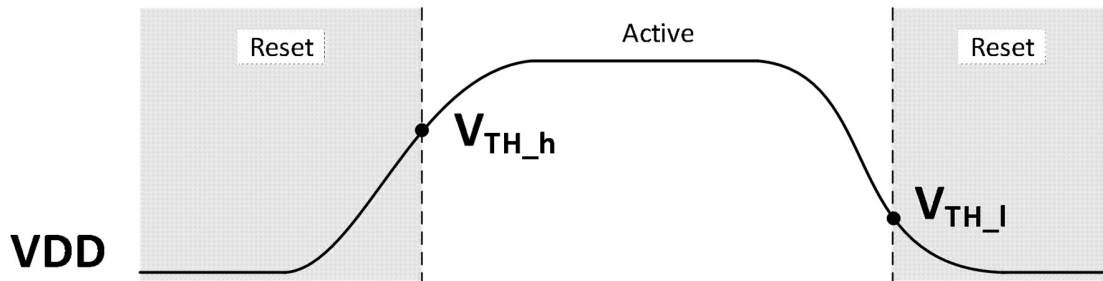
Figure 11: UVLO reset
