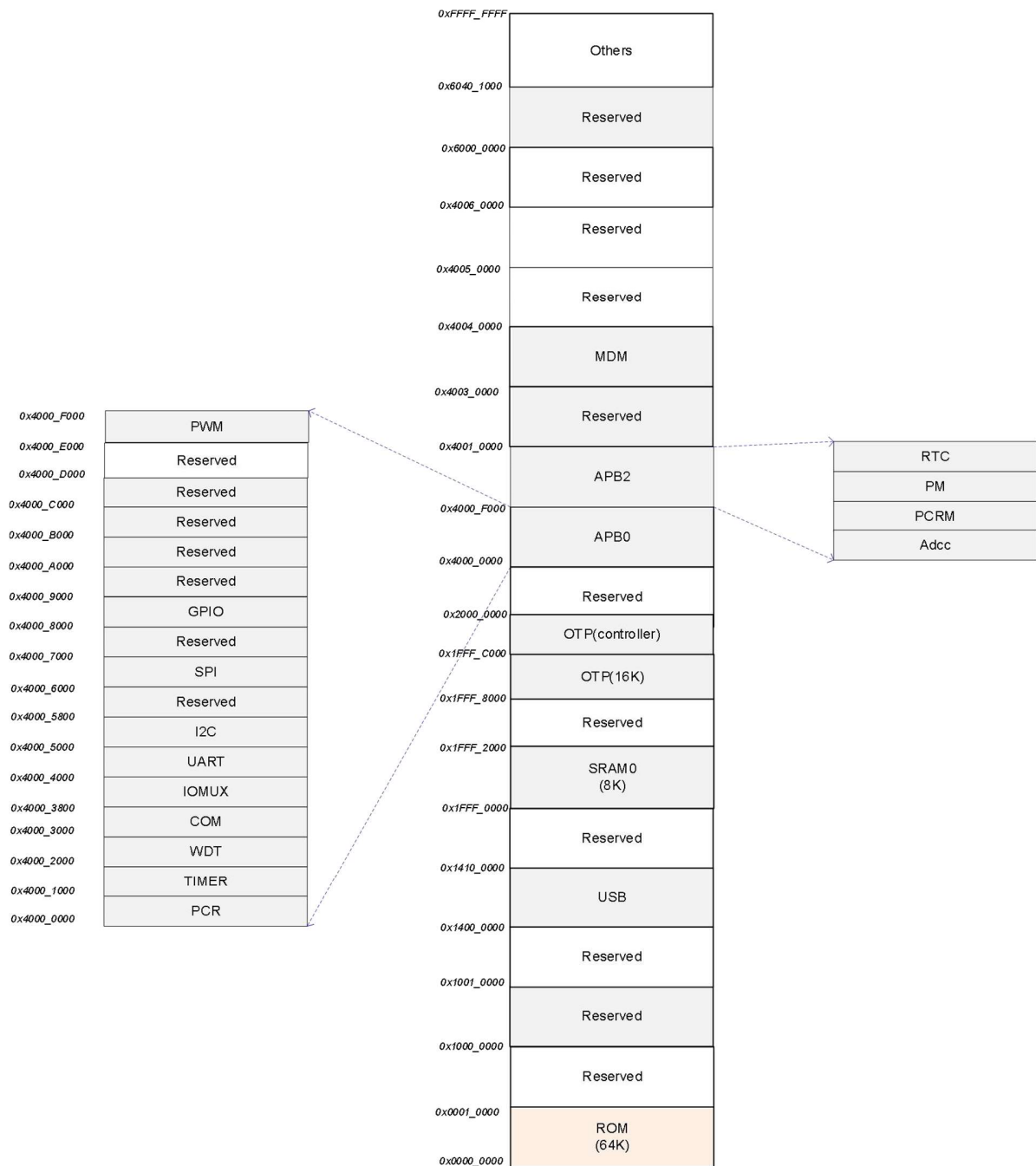
Figure 7: WL2630 Memory Space
