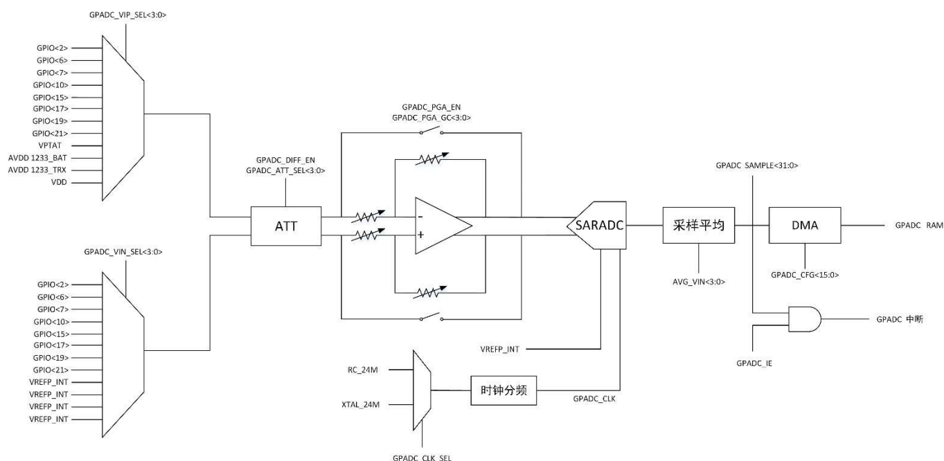
Figure 13.1 GPADC 框图
