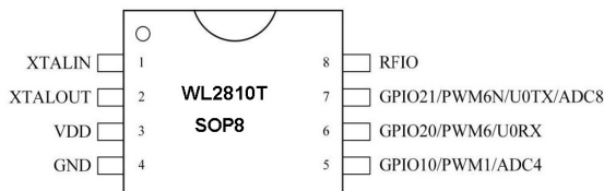
Figure 1-4 SOP8 封装图
