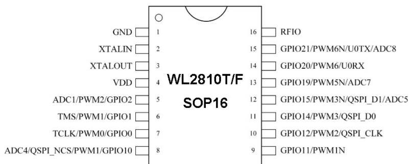
Figure 1-2 SOP16 封装图
