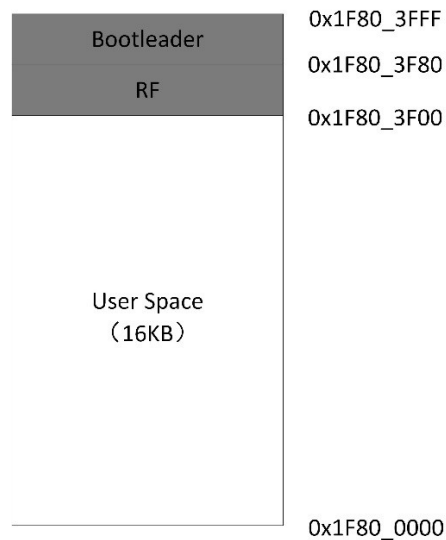
Figure 5-1 OTP Memory Map
